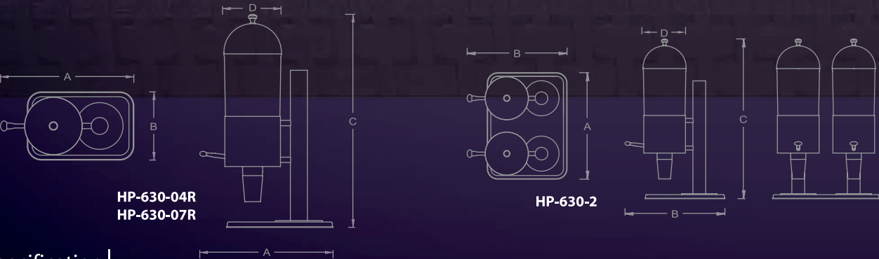
Flow adjuster to allow dispensing various types of cereals
