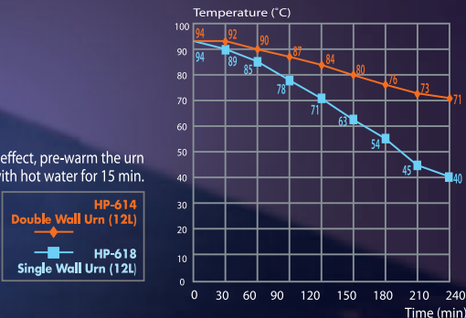
Heat loss rate of coffee urn (12L) - at room temperature 22 °C
